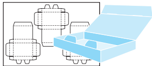
Playing Card Box 3-up 2.5 x 3.625 x .75
