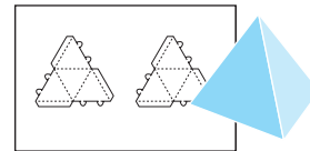
Pyramid Box 2-up 3.05 x 3.05 x 2.39
