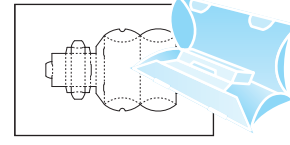
Flash Drive Mailer 1-up 5 x 3 x 1.875
