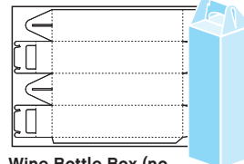
Wine Bottle Box (no window) 1-up 3.375 x 13.25 x 3.375
