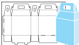
Lunch Box 1-up 6.25 x 6.125 x 2.375
